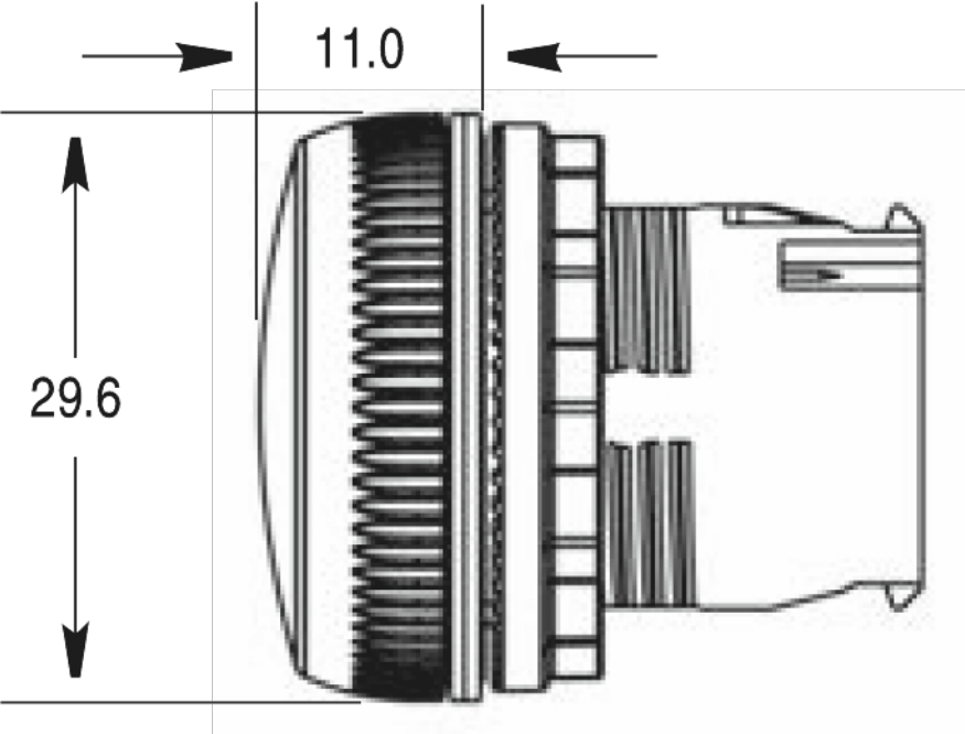
Dimension Diagram
